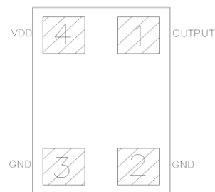
Pin configuration (Bottom view)
