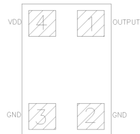
Pin configuration (Bottom view)
